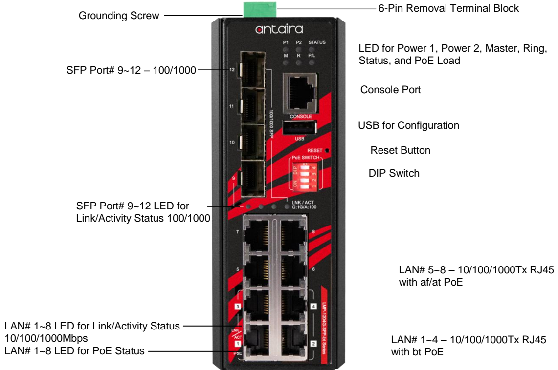
Figure 2.2 - The Front Panel of LMP-1204G-SFP-bt Series
