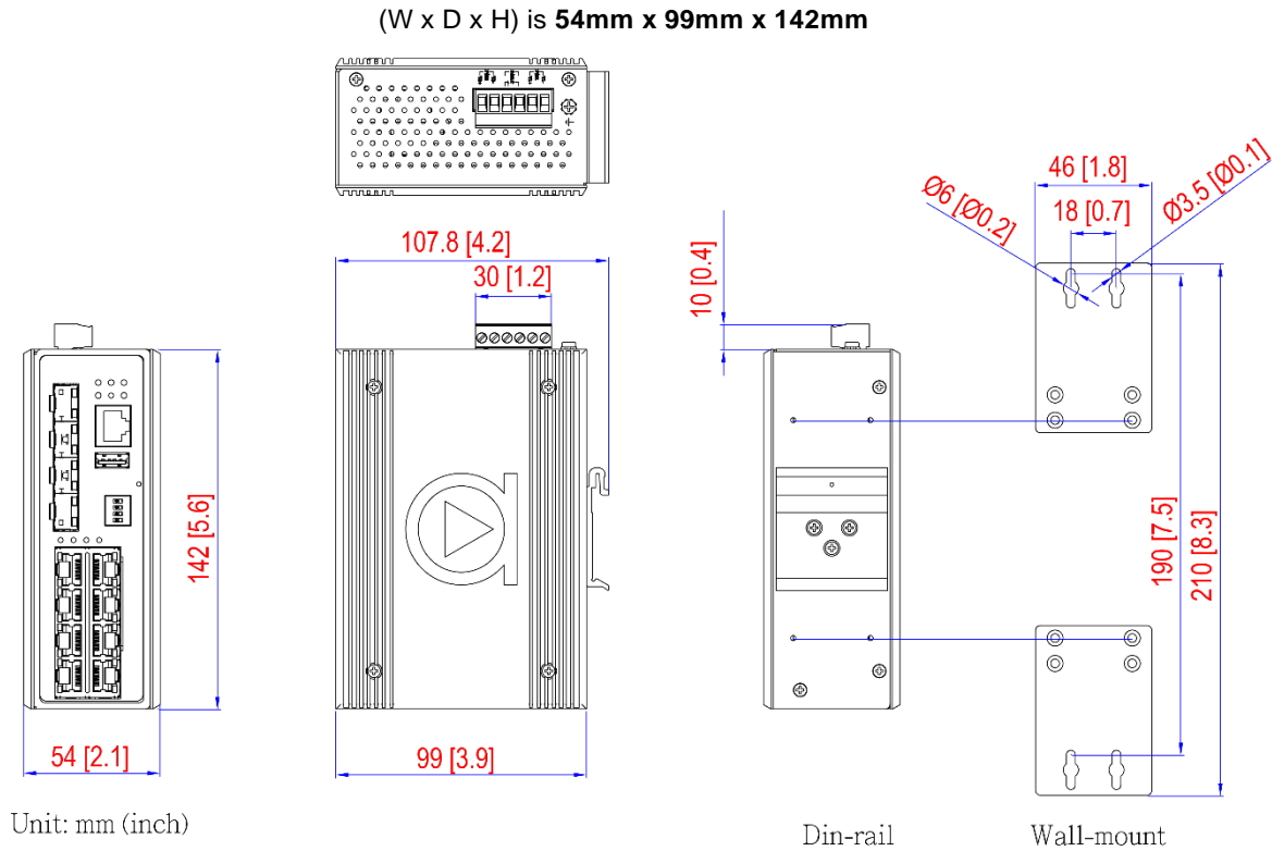
Figure 2.1 LMP-1204G-SFP-bt Series Physical Dimensions
