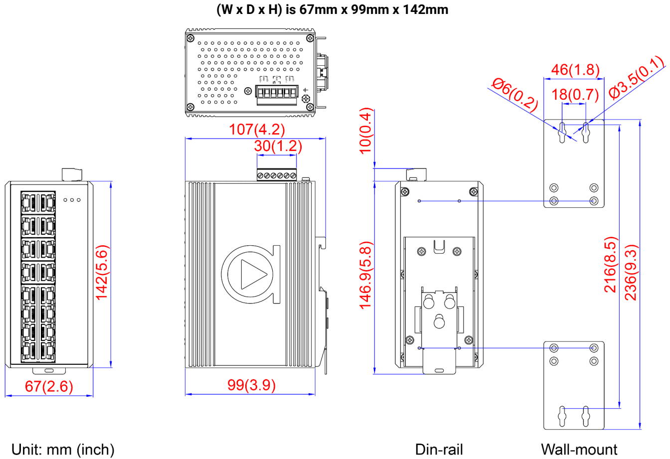
Figure 2.1 - Physical Dimensions
