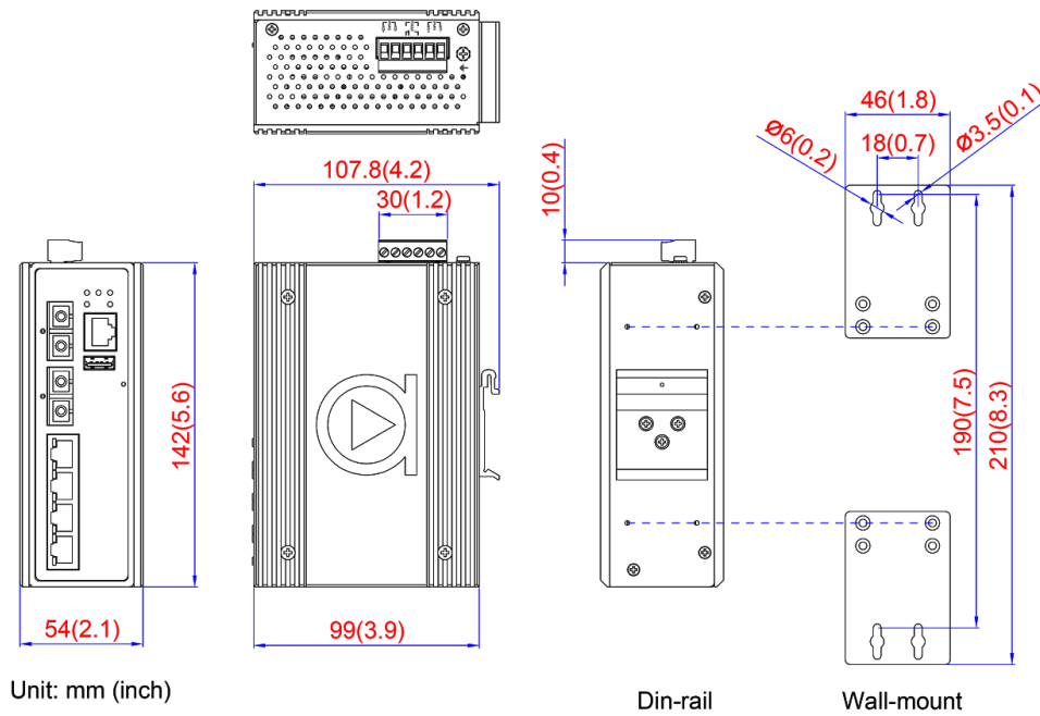
Figure 2.1 - Physical Dimensions
