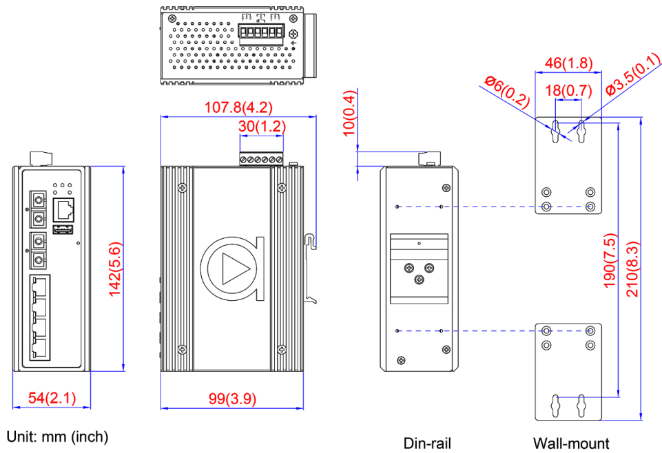
Figure 2.1 - Physical Dimensions
